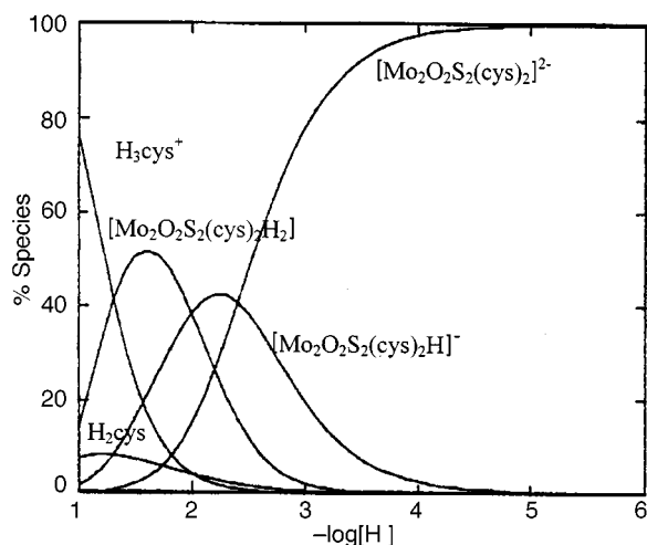
Fig. 4 Species distribution diagram as a function of -\log[H^+] for [\text{Mo}_2\text{O}_2(\mu\text{-S})_2(\text{cys})_2]^{2-} \times 3 \times 10^{-3} \text{ mol dm}^{-3} , using cysteine as reference
