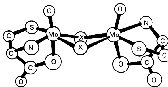
Fig. 1 Structure of the \text{Mo}^{\text{V}}_2 complexes [\text{Mo}_2\text{O}_2(\mu\text{-X})_2(\text{cys})_2]^{2-} , \text{X} = \text{O} or \text{S} . 4,8
